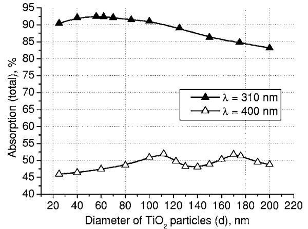
Fig. 8 Absorption within the whole horny layer (20- \mu m-thick) for the light of 310 (▲) and 400 nm (△). The volume concentration of TiO 2 particles is 5%.
