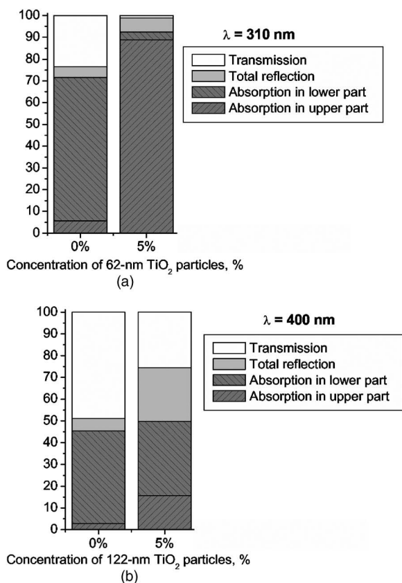
Fig. 10 Effect of the “best” TiO 2 particles [sizes of (a) 62 and (b) 122 nm] distributed homogeneously within the 1- \mu m-thick upper part (volume concentration 5%) of the 20- \mu m-thick horny layer for (a) 310- and (b) 400-nm light.
