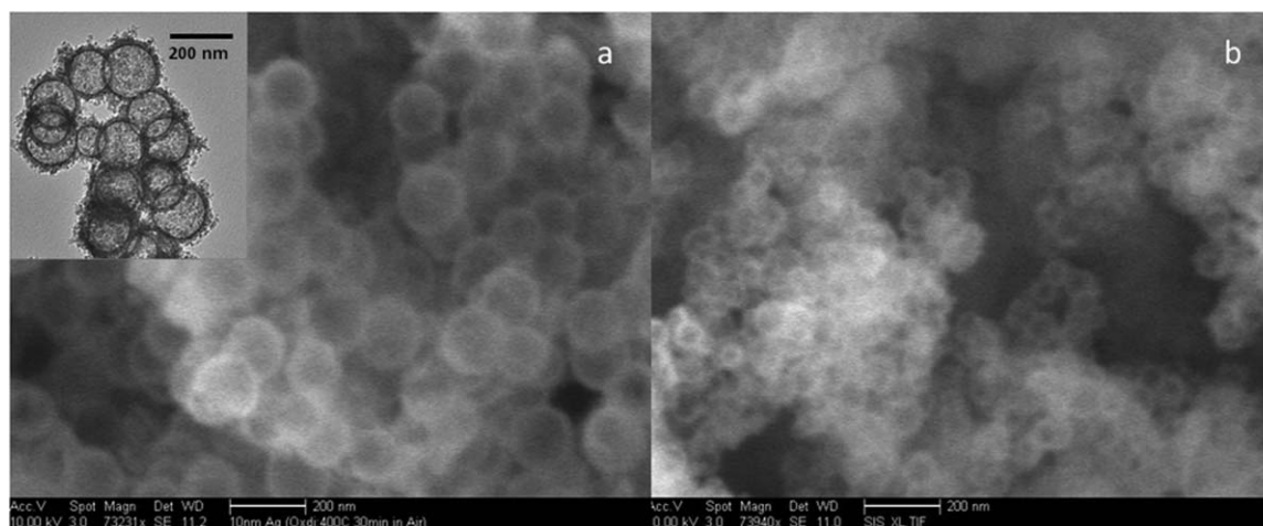
Fig. 1 SEM and TEM images of europium doped silica nanoshells from (a) 200 and (b) 100 nm APS templates with europium of 0.54 and 1.35% mole, respectively. Scale bars in SEM and TEM images are 200 nm.
