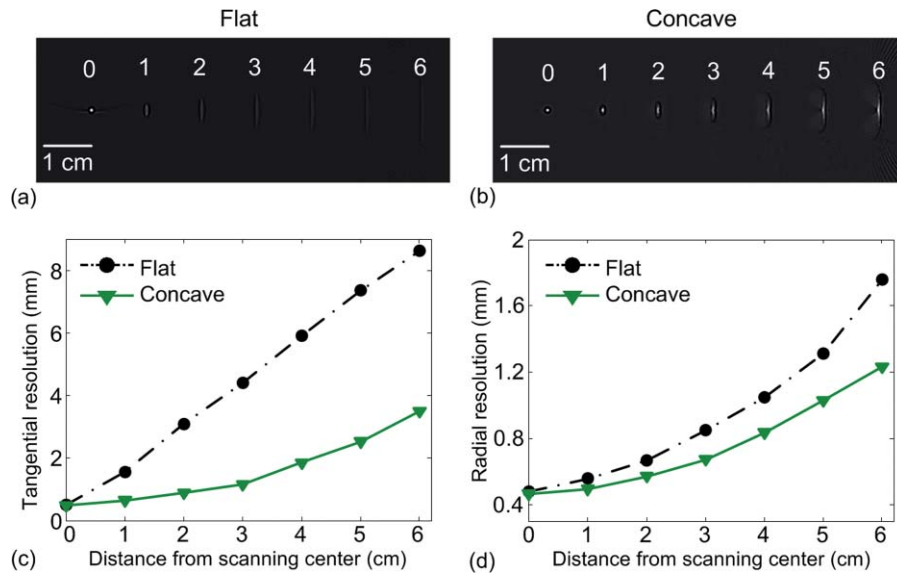
Fig. 3 Simulation results of the resolutions versus distance from the scanning center. Reconstructed PAT image of seven point targets acquired with (a) the flat transducer, and (b) the concave virtual point detector. (c) Tangential resolution and (d) radial resolution versus distance from the scanning center.
