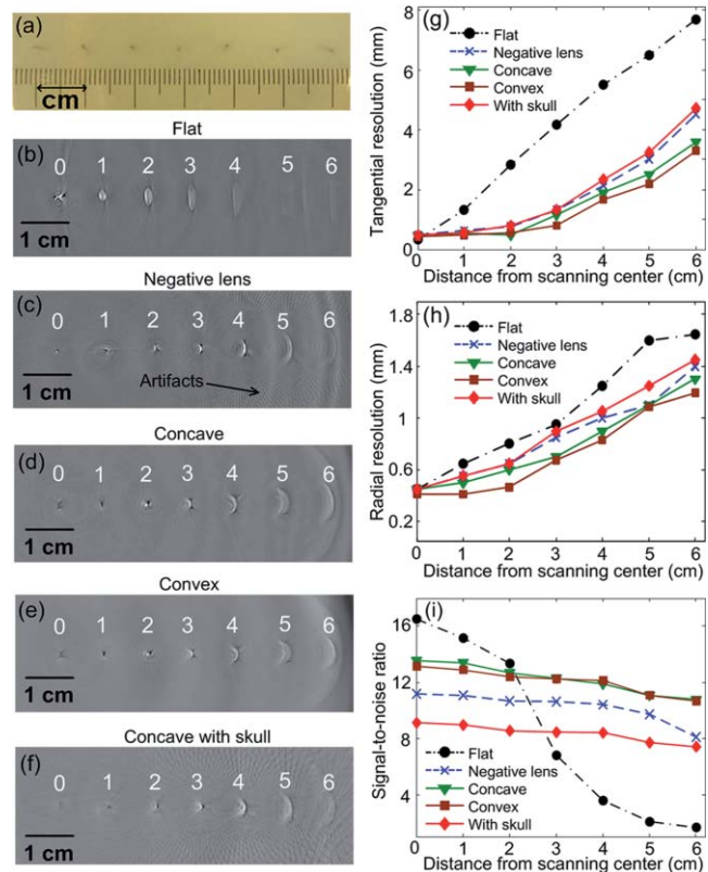
Fig. 4 PAT of needles and the resolution and SNR quantifications. (a) Photograph of seven needles inserted in agar at different distances from the scanning center. PAT of the phantom acquired with (b) a flat transducer, (c) a negative-lens transducer, (d) a concave virtual point transducer, (e) a convex virtual point transducer, and (f) a virtual point detector with the phantom enclosed by a monkey skull. Quantification of (g) tangential resolution, (h) radial resolution, and (i) SNR of the PAT systems versus distance from the scanning center.
