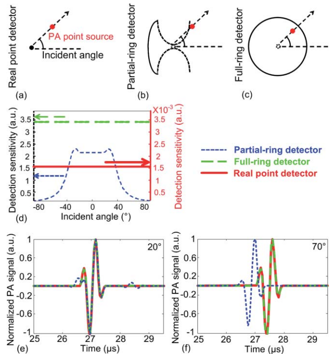
Fig. 2 Comparison of a real point detector, a partial-ring detector, and a full-ring detector. Schematics of the PA signal detection mode of (a) a real point detector, (b) a partial-ring detector, and (c) a full-ring detector. (d) Detection sensitivity distributions versus incident angle for the three detectors. Normalized PA signals from the point source acquired with the three detectors at the (e) 20 deg incident angle and (f) 70 deg incident angle.
