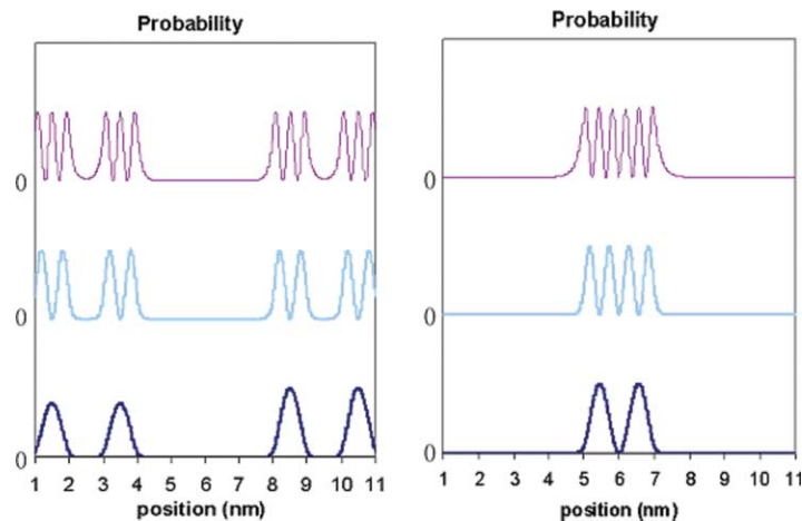
Fig. 8 Electron density of probability in a nonperiodic structure composed of five coupled wells of depth 2.9 eV, of widths 1, 1, 2, 1, and 1 nm, respectively. The distance between each well is 1 nm.
