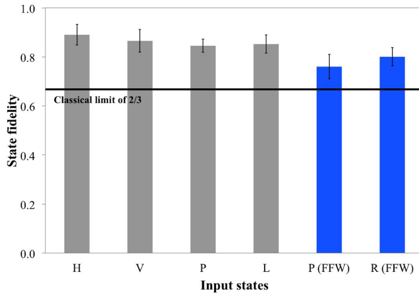
Fig. 4. Experimental results of the teleported state fidelities for first part (grey) without feed-forward (FFW) and second part (blue) with FFW. All observed fidelities are clearly above the classical limit of 2/3 . Error bars are plus/minus 1 sigma, assuming Poissonian statistics.
