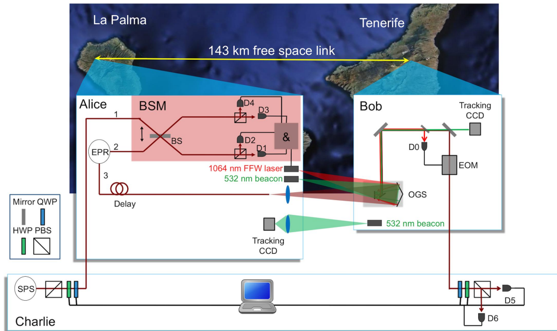
Fig. 3. Scheme of the 143 km free-space quantum-teleportation experiment between the Canary Islands La Palma and Tenerife. Charlie prepares the input state (photon 1) from a single-photon source (SPS) to be teleported on photon 3. Alice then performs a Bell-state measurement (BSM) on photons 1 and 2, where photon 2 is from the entangled photon pair 2 and 3 of the Einstein-Podolsky-Rosen (EPR) pair source. Photon 3 gets delayed until the outcome of the BSM has been transmitted to Bob via a classical laser pulse of 1064 nm wavelength. Bob prepares the electro-optical modulator (EOM) to perform the corresponding unitary transformation on photon 3 and measures its polarization state by means of a quarter-wave plate (QWP), a half-wave plate (HWP) and a polarizing beam splitter (PBS). A bidirectional tracking system based on beacon lasers with 532 nm wavelengths and tracking CCD cameras on both sides is used to enhance the link stability.
