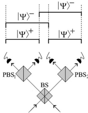
Fig. 2. The Bell-state measurement (BSM) projects photon 1 and 2 onto the four Bell-states with equal probability of 1/4. Experimentally only two states can be resolved with linear optics only. Simultaneous clicks in the first and third detector (from the left) or the second and fourth detector indicate the projection on the |\Psi^- \rangle_{12} Bell-state, whereas if detectors one and two or three and four click simultaneously a |\Psi^+ \rangle_{12} Bell-state is detected.
