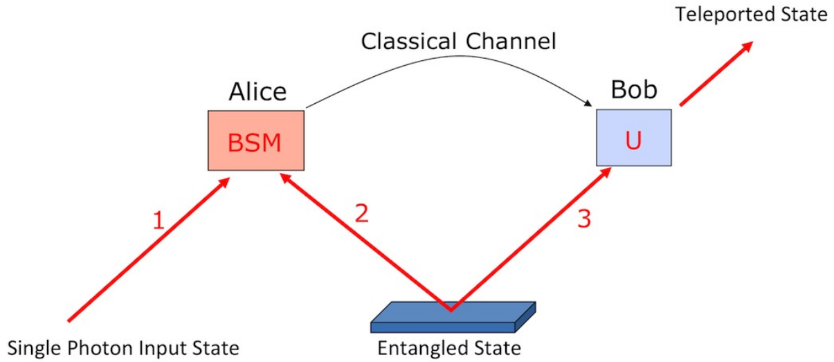
Fig. 1. Schematics of the quantum-teleportation protocol [8].
