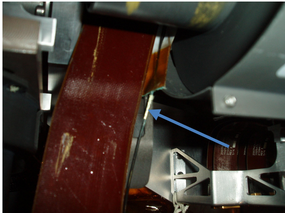
Fig 3 Separated outer jacket in motion life test. The arrow points to the kevlar braid strength member in the cable that was exposed after the jacket separated.
