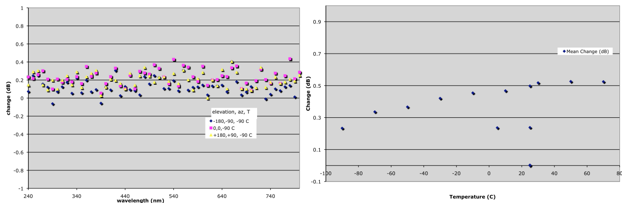
Fig 4 Change in attenuation vs temperature and position angle at -90 C and three different sets of azimuth and elevation angles, referenced to +25 C and 0 elevation, 0 azimuth (left). Mean change over all wavelengths vs temperature at 0 elevation and 0 azimuth (right). See text for explanation of the trend.
