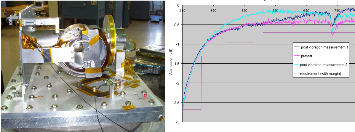
Fig 2 RSM thermal and mechanical simulator (left) and attenuation data from vibration testing (right)
