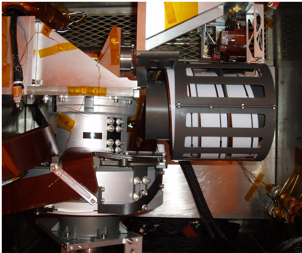
Fig. 1. The mechanical mockup of the MSL Remote Sensing Mast used for testing the ChemCam fiber optic cable in motion. The mockup accurately copies the interfaces and motions of the RSM and the optical fiber.
