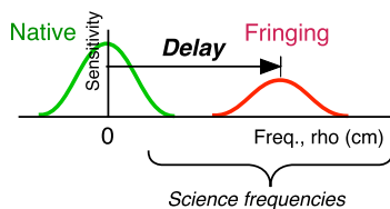
Fig. 3 Heterodyning shifts the native spectrograph sensitivity peak from zero to a higher frequency, where science frequencies typically reside, by the interferometer delay \tau , and to 50% amplitude. Frequency in units of features per wavenumber ( \text{cm}^{-1} ) conveniently has units of delay (cm).
