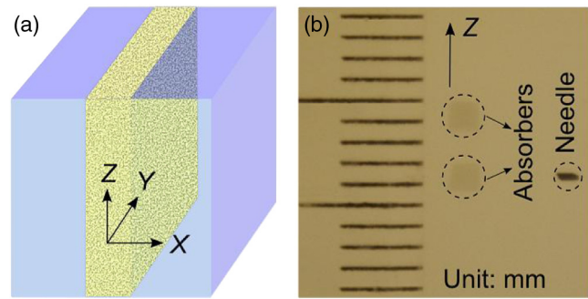
Fig. 2 Tissue-mimicking phantom to be imaged. (a) The dimensions of the phantom are 4 \times 8 \times 8 \text{ cm}^3 ( X \times Y \times Z ). A 5-mm-thick scattering layer with reduced scattering coefficient \mu'_s = 6 \text{ cm}^{-1} was sandwiched between two transparent gelatin gel layers. (b) In the mid-X plane of the scattering layer, two optical absorbers and a needle were embedded. The two absorbers were made by infusing optically absorbing India ink. The needle was used to align the two ultrasonic transducers with respect to the two absorbers.
