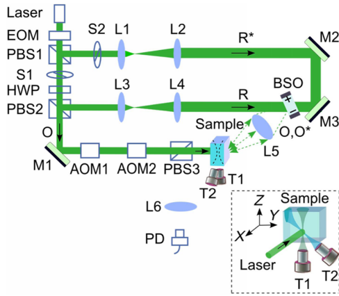
Fig. 1 Schematic of the experimental setup. AOM, acousto-optic modulator; BSO, \text{Bi}_{12}\text{SiO}_{20} ; EOM, electro-optic modulator; HWP, half-wave plate; L, lens; M, mirror; O, signal light; O^* , time-reversed signal light; PBS, polarizing beam splitter; PD, photodiode; R, reference beam; R^* , conjugated reference beam; S, shutter; T, ultrasound transducer. Coordinates: X = optical axis, and Z = acoustic axis of T1. The pressure at the ultrasound focus was 1.0 MPa peak-to-peak. To enhance the phase conjugation efficiency, a 2.1-kHz, 8-kV pp square waveform external electric field was applied across the BSO.
