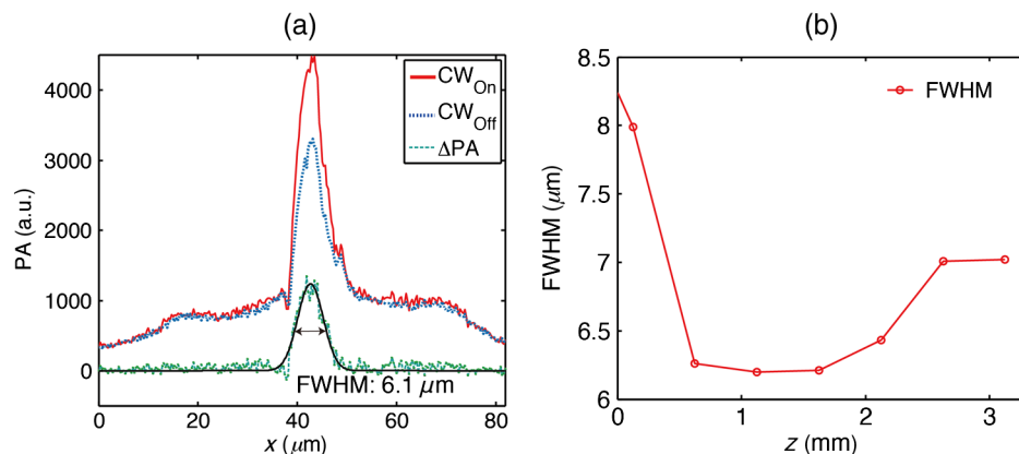
Fig. 3 Cross-sectional images of a 6\text{-}\mu\text{m} -diameter carbon fiber. (a) Red line: one-dimensional (1-D) photoacoustic (PA) image acquired when the CW laser is on. Blue line: 1-D PA image acquired when the CW laser is off. Green line: the differential PA image \Delta\text{PA} . Black line: Gaussian fit of \Delta\text{PA} . The FWHM of the \Delta\text{PA} image is 6.1\text{ }\mu\text{m} . To improve SNR, 20 measurements were averaged. (b) Axial distribution of the FWHM of the cross-sectional carbon fiber images. The axial coordinate z is relative to the beginning measurement position ( z = 0 is about 7\text{ mm} away from the tip of the axicon lens).
